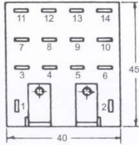
SCHEMATIC DIAGRAM OF RE BASE PLATE
