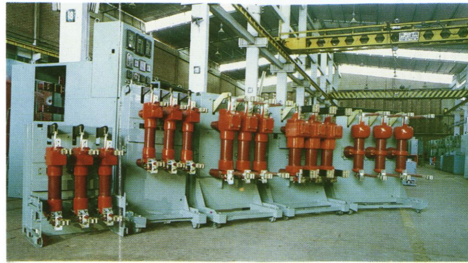
Range of MOCBs
